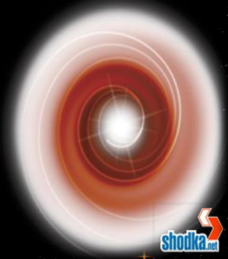
Neutron Star X-ray Nova
