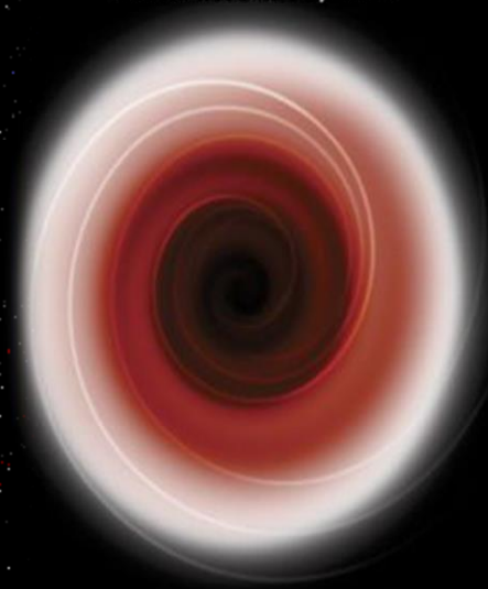
Black Hole X-ray Nova
